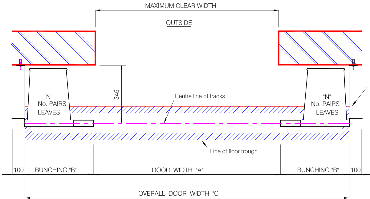
PLAN VIEW
