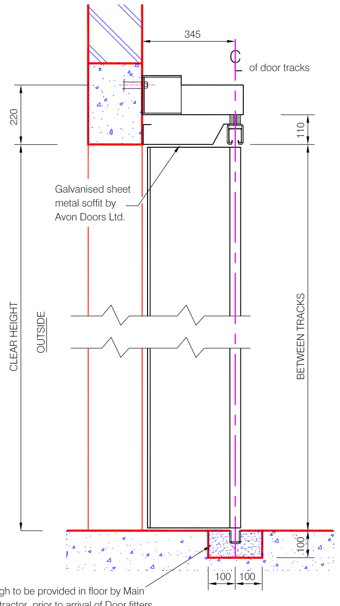
SECTION
